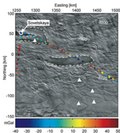
Figure 2: Detail of ice surface revealing outline of 90°E lake (center) and part of Sovetskaya Lake (beneath Sovetskaya research station). Data from 1958 Soviet study (colored dots) revealed a noticeable drop in the Earth's gravitational pull above the two lakes. White triangles mark the locations of smaller lakes beneath the ice.
