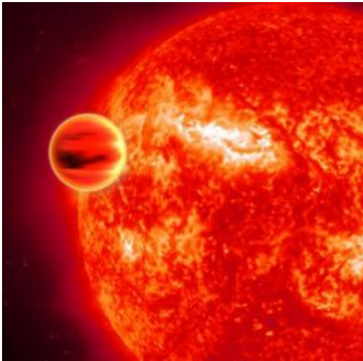
An artist's impression of HD 189733b and its star as though viewed using infrared. Credit: ESA - C. Carreau
