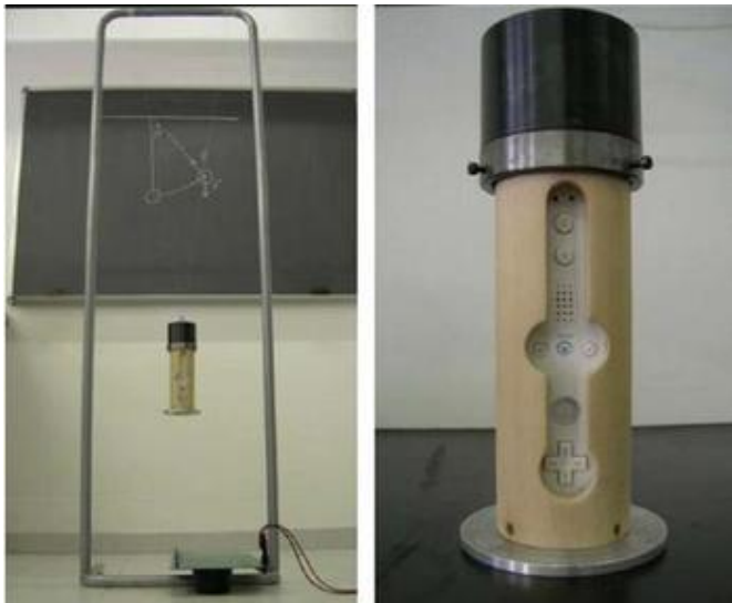
Wii accelerometer as a pendulum. Image credit: Vannoni and Straulino.
