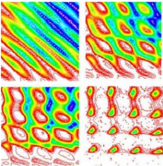
The colorized images show how tuning the voltage of the three gates controls very small amounts of electrical charge and regulates current flow in the new silicon transistor. In the first figure, the pattern of diagonal lines indicates the charge is correlated throughout the device, and current is flowing (at levels ranging from 0 Amps shown in red, to 1.4 nanoAmps shown in violet). The next three figures show what happens as the voltage applied to the center gate is reduced. In the last figure, the square pattern indicates the charge has separated in the device, and the large amount of white space indicates a related drop off in the current. Credit: NTT/NIST
