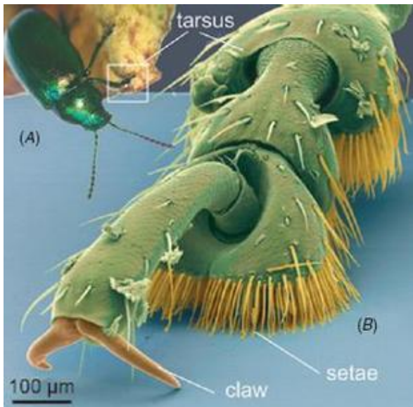
(A) Chrysomelid beetle with (B) a close-up of the tarsus with a hairy adhesive system (colored scanning electron microscope image).
