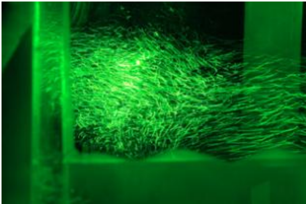
Particles (in false color) seen as they move in turbulent water, viewed in a time-lapse photograph.
