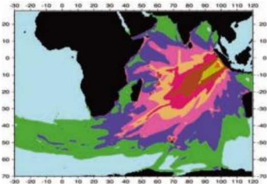
Tsunami propagation pattern from earthquake west of Sumatra island, Indonesia. Credit: USC Tsunami Research Center/Northwestern University
