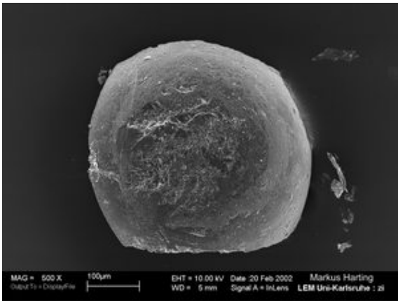
Scanning Electron Microscope picture of isolated, and well preserved Spherule from NE-Mexico (400 µm in diameter).
