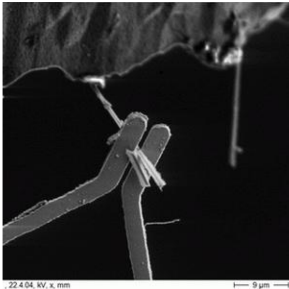
Pulling a nanowire from its substrate.
