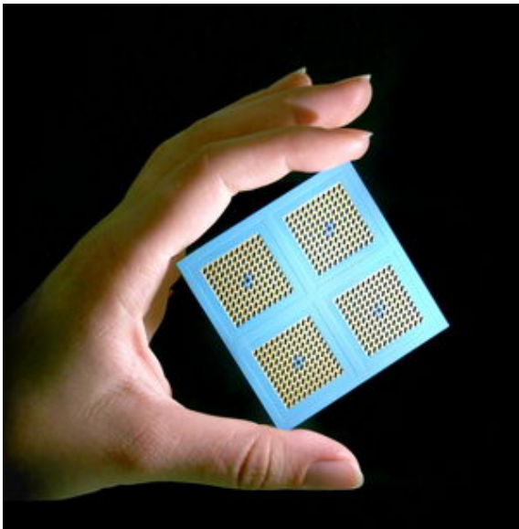
Integrated ceramic micro fuel cell system for portable applications. © Fraunhofer IKTS
