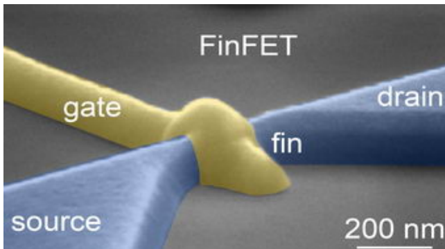
Electronmicroscopic image of FinFET transistor that was used for the research. Credit: TU Delft
