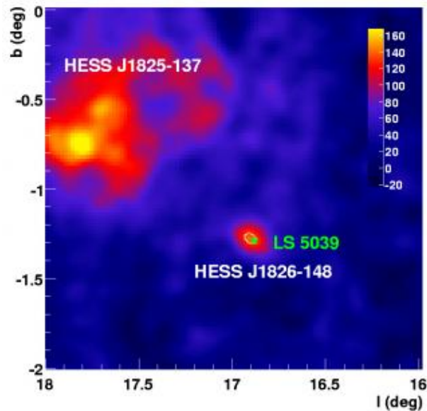
Map of the gamma ray sky in the region of LS5039. The green star shows the position of LS5039 as measured using radio telescopes and the white ellipse shows the gamma ray position. Credit: PPARC
