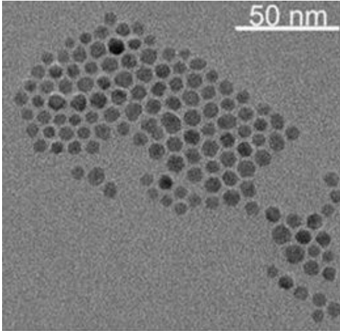
Electron microscopy of the magnetic nanoparticles. Credit: IMEC
