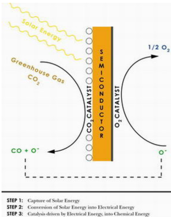
Graphic depicting steps in solar splitting of CO 2 . Credit: Aaron Sathrum, UCSD
