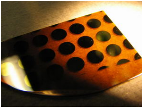
CO 2 splitting semiconductor/catalyst device under construction (gallium phosphide wafer with metal contacts) Credit: Aaron Sathrum, UCSD
