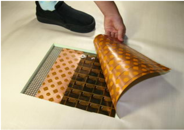
The wireless power transmission sheet, shown embedded into a floor. Credit: Takao Someya
